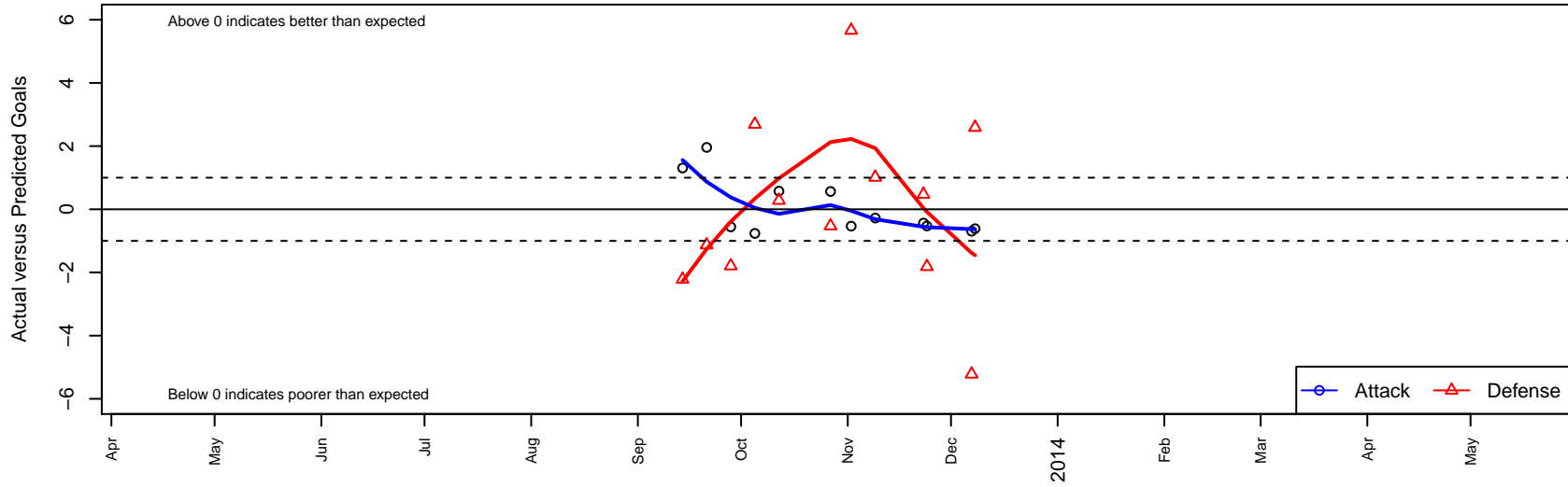
Highline Premier 01-00 B00 Dots are actual minus expected GF (blue circles) and GA (red triangles). Blue line is smoothed change in attack strength. Red is smoothed change in defense strength.
